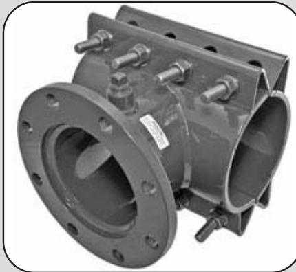
632 Tapping Sleeve
